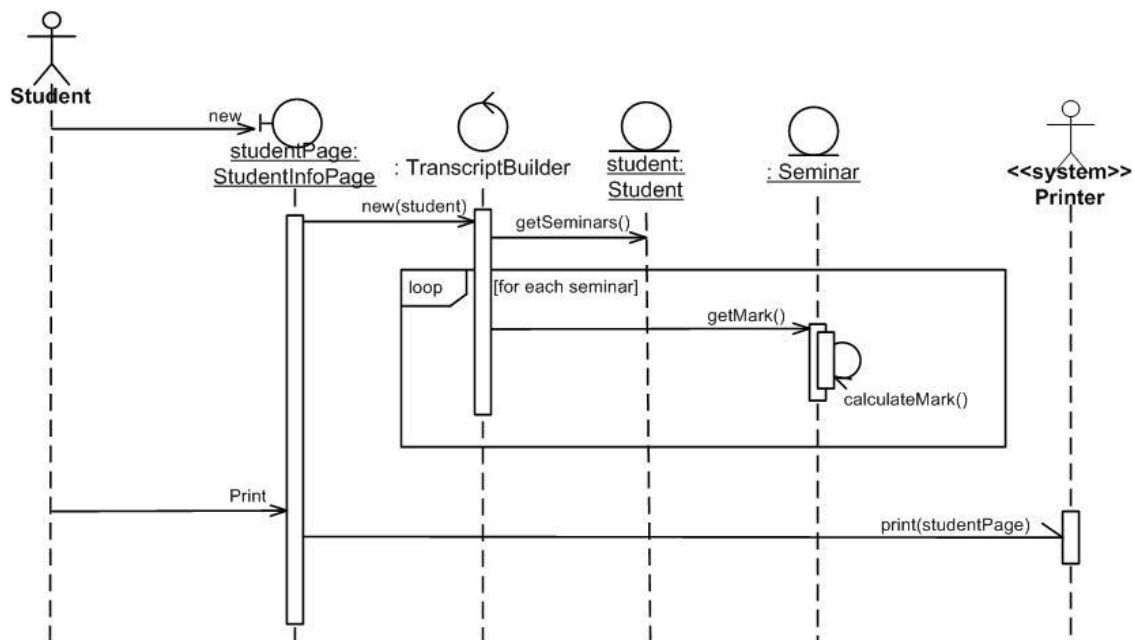
Figure 6. Outputting transcripts.
