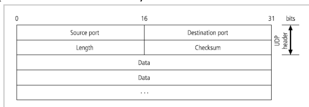
Figure 6-4 UDP Datagram Structure
