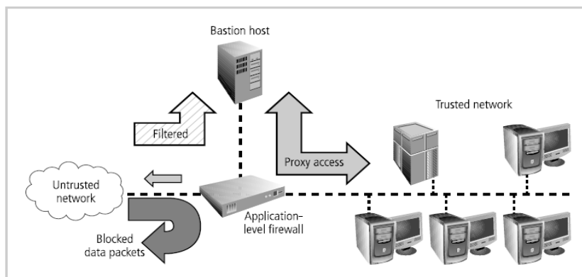
Figure 6-12 Screened Host Firewall
