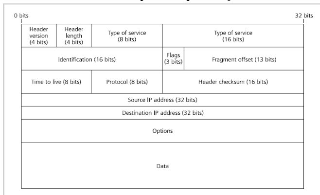
Figure 6-2 IP Packet Structure
