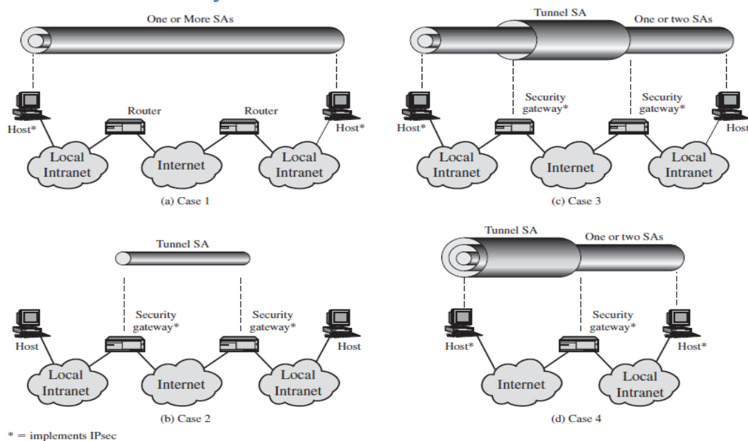
Figure 8.10 Basic Combinations of Security Associations
