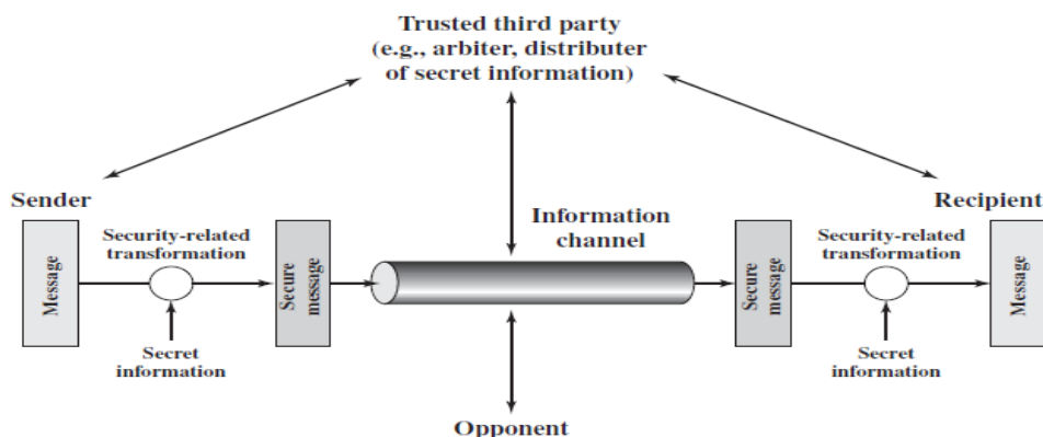
Figure 1.4 Model for Network Security
