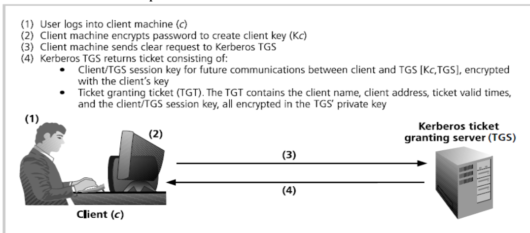
Figure 6-17 Kerberos Login
