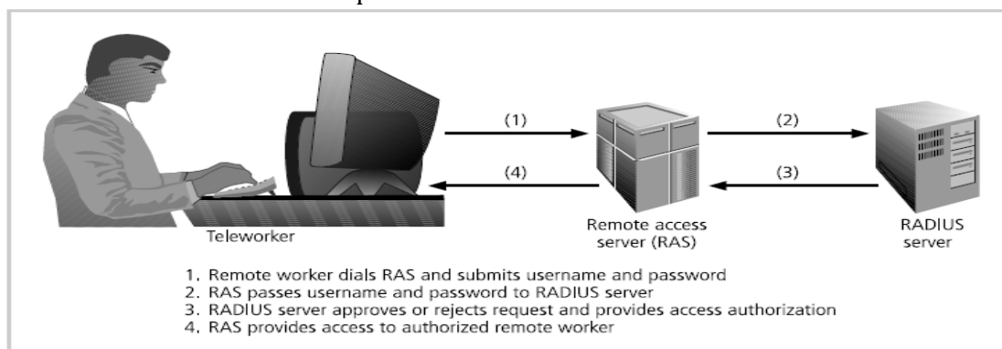
Figure 6-16 RADIUS Configuration
