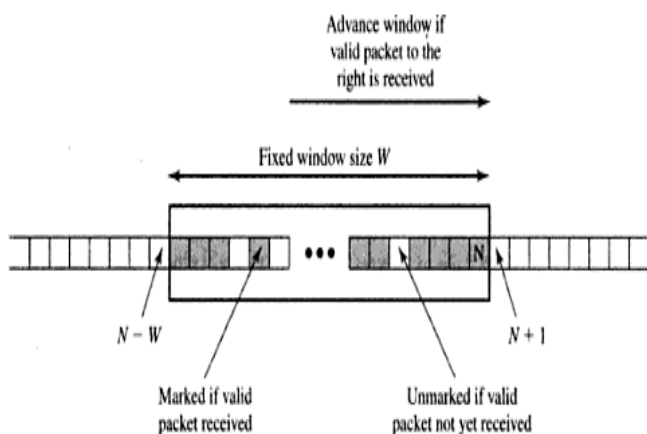
Figure 6.4 Antireplay Mechanism
