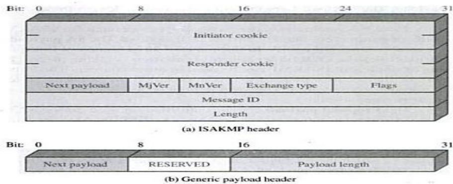
Figure 6.12 ISAKMP Formats
