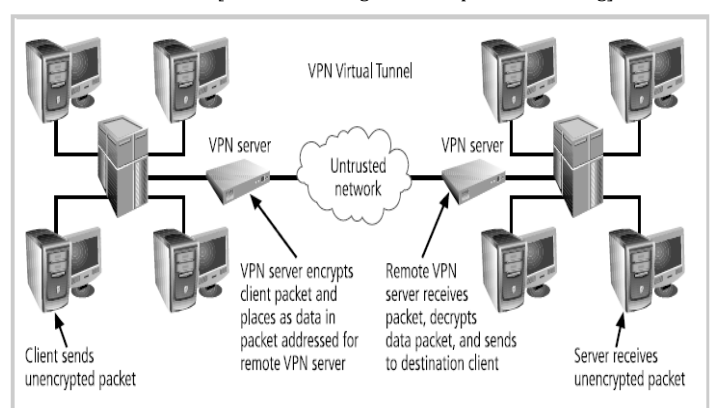
Figure 6-20 Tunnel Mode VPN
