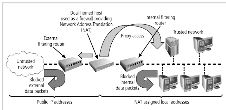
Figure 6-13 Dual-Homed Host Firewall
