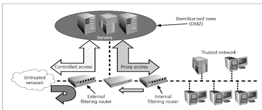
Figure 6-14 Screened Subnet (DMZ)
