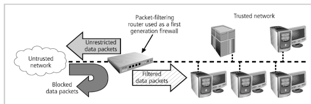
Figure 6-5 Packet-Filtering Router
