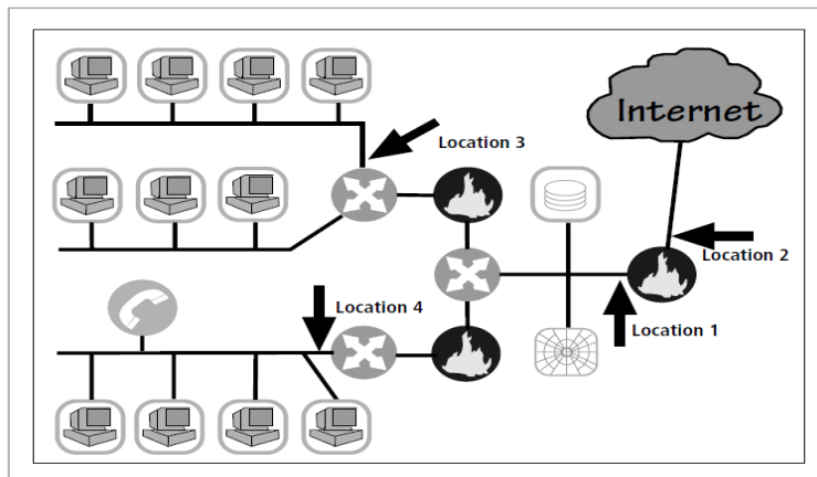
Figure 7-7 Network IDPS Sensor Locations 17
