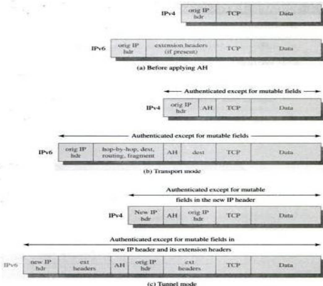
Figure 6.6 Scope of AH Authentication
