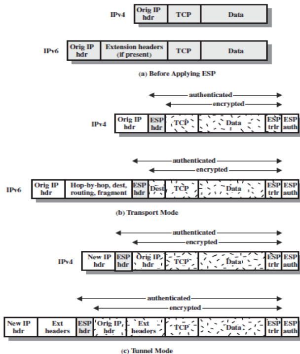
Figure 8.8 Scope of ESP Encryption and Authentication
